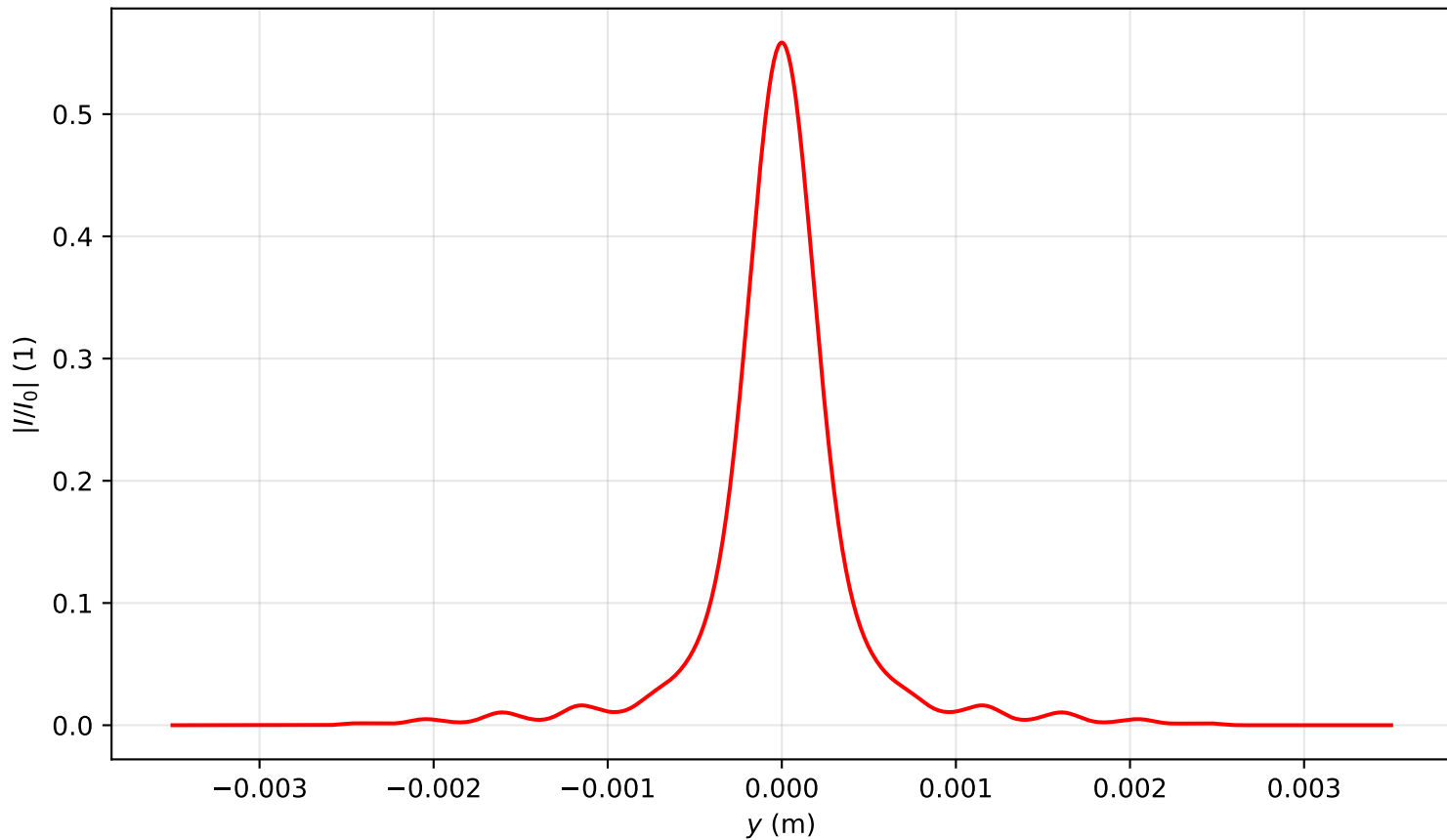
Intensity profile I(x = 0, y, z = 3.025)/I_0 , P_{in}=3.0P_{cr} , artificial time
